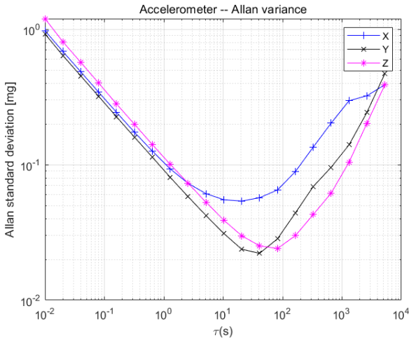
Figure3: CH010 Accelerometer Allan Variance
