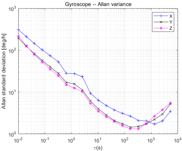
Figure8: CH040 Gyroscope Allan Variance
