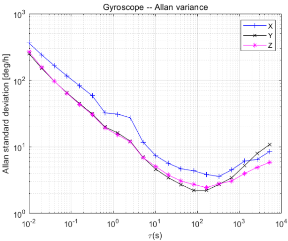
Figure6: CH020 Gyroscope Allan Variance
