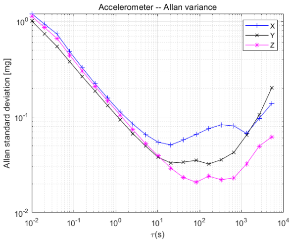
Figure5: CH020 Accelerometer Allan Variance
