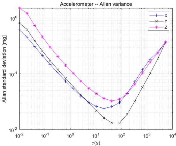
Figure7: CH040 Accelerometer Allan Variance
