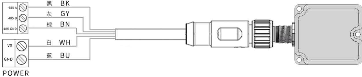
Figure 25: M12-A code 5pin to open RS-485
