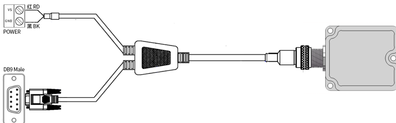
Figure 20: M12-A code 5pin to DB9+OPEN external power RS-232
