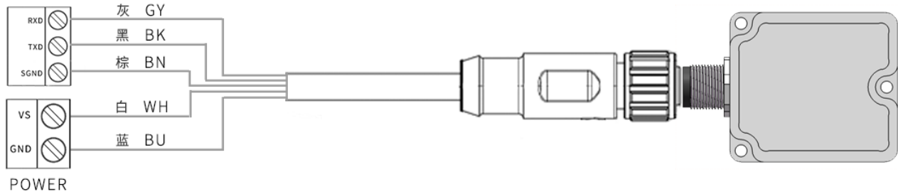
Figure 27: M12-A Code 5pin to Open UART
