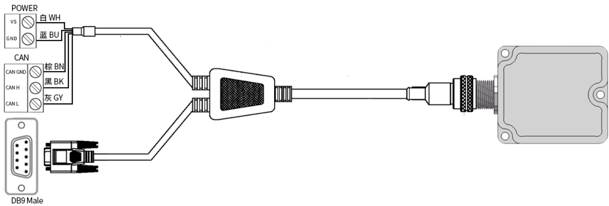
Figure 23: M12-A code 8pin to DB9+OPEN external power CAN+RS-232
