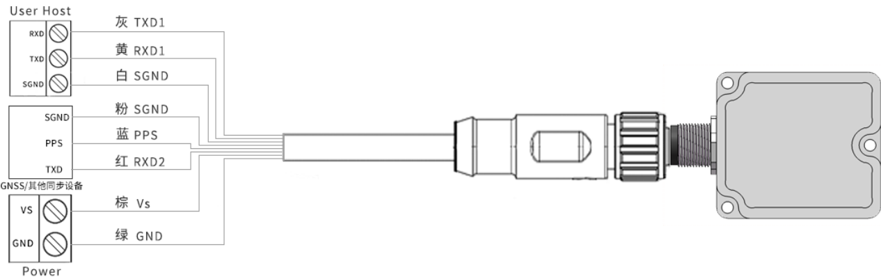
Figure 30: PPS+UTC Synchronous
