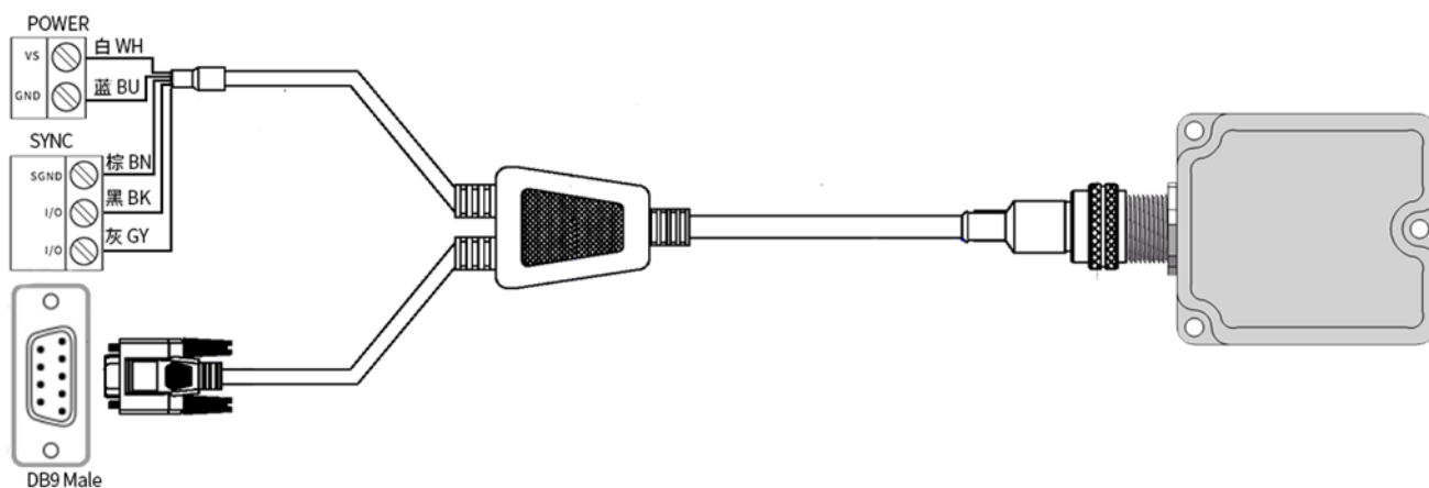
Figure 21: M12-A code 8pin to DB9+OPEN
