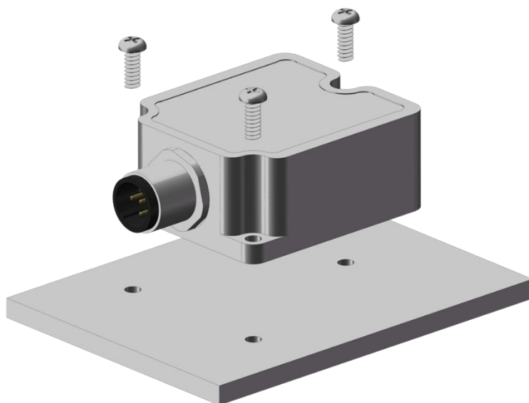
Figure 32: Mounting Example
