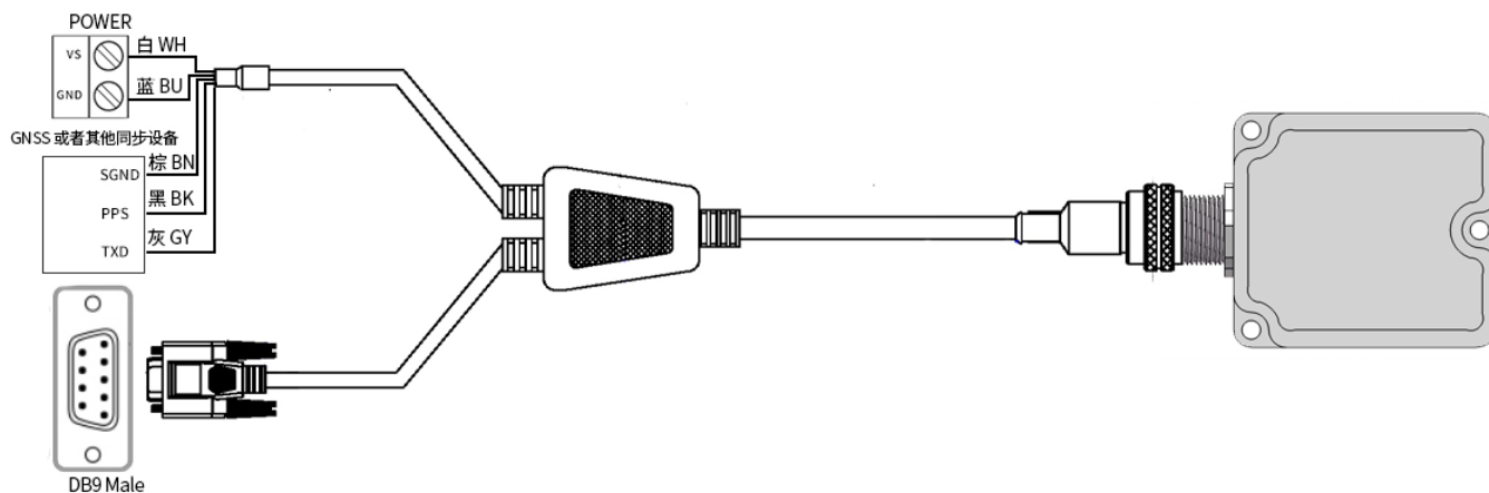
Figure 22: M12-A code 8pin to DB9+OPEN PPS+UTC
