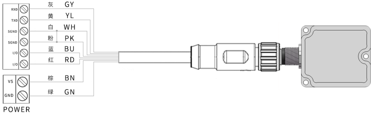
Figure 28: Synchronous with UART common ground
