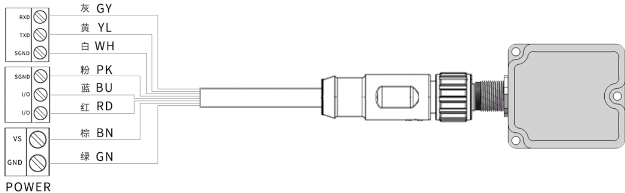
Figure 29: Synchronous with UART not common ground
