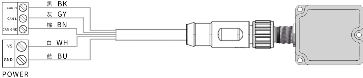
Figure 26: M12-A code 5pin to open CAN
