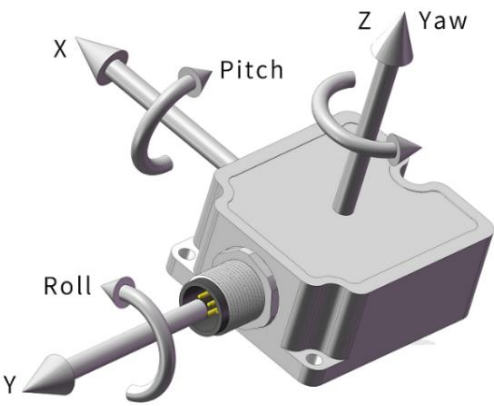
Figure 31: Coordinate System
