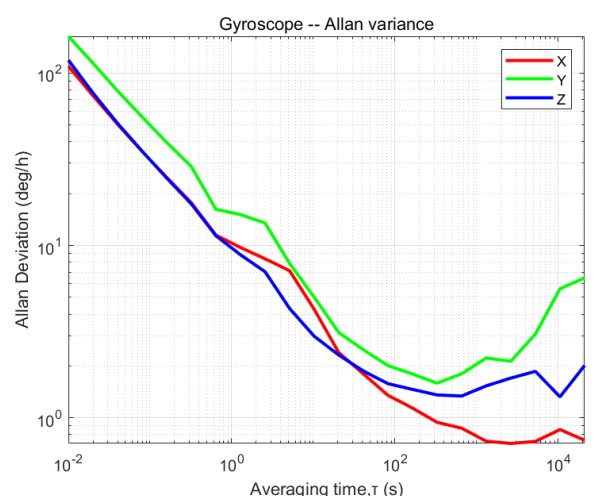
Figure 8: HI14R5 Gyroscope Allan Variance
