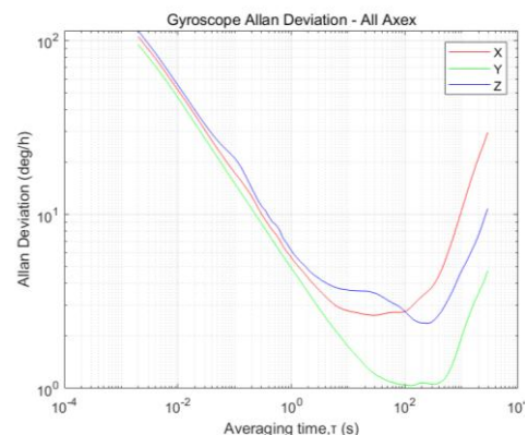
Figure12: HI05RX Gyroscope Allan Variance
