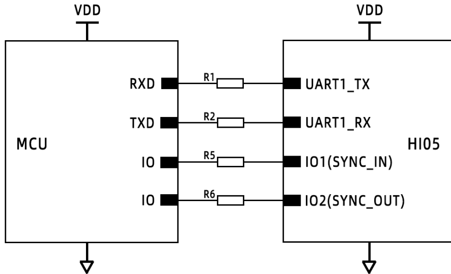
Figure9: HI05 UART communication with synchronization
