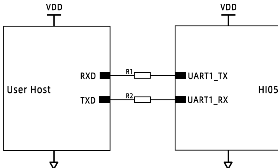
Figure6: HI05 UART communication ceference circuit
