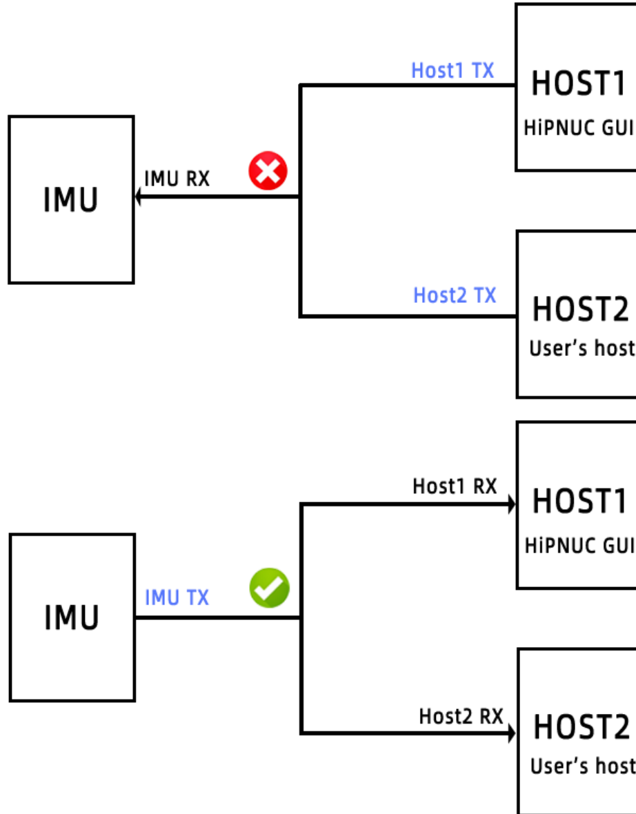
Figure26: IMU serial port simultaneously connected to the user's host and HiPNUC GUI
