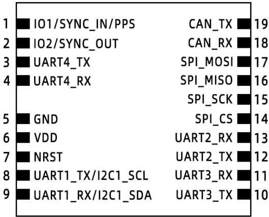
Figure3: HI05XX-MI0 pin assignment
