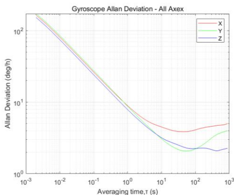
Figure11: HI05MX Gyroscope Allan Variance
