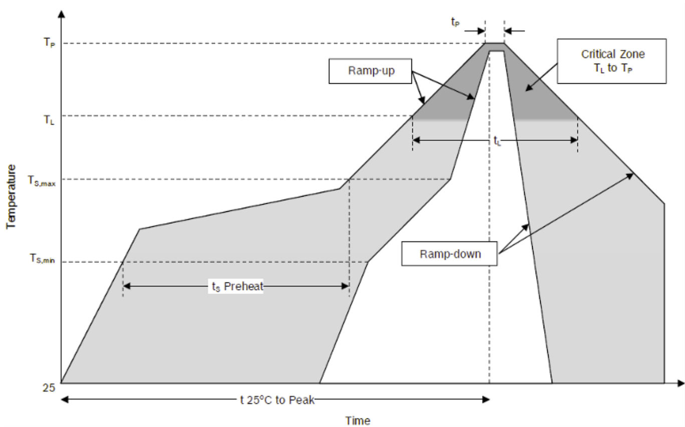
Figure21: SMT temperature curve
