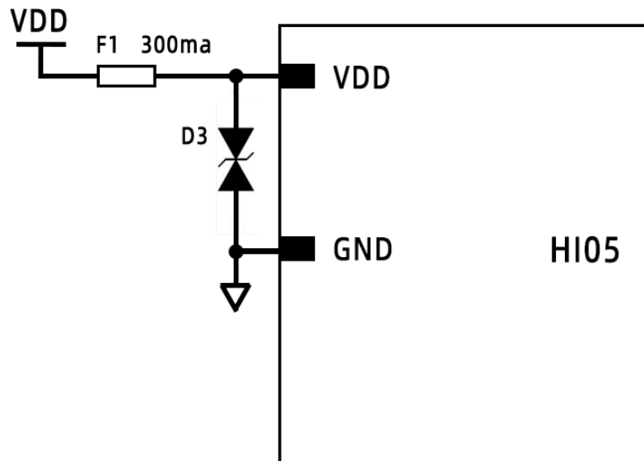
Figure5: HI05 UART communication reference circuit
