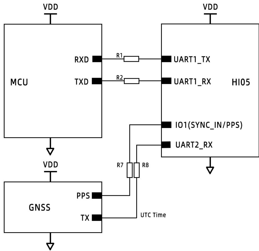
Figure10: HI05 GNSS-based synchronization
