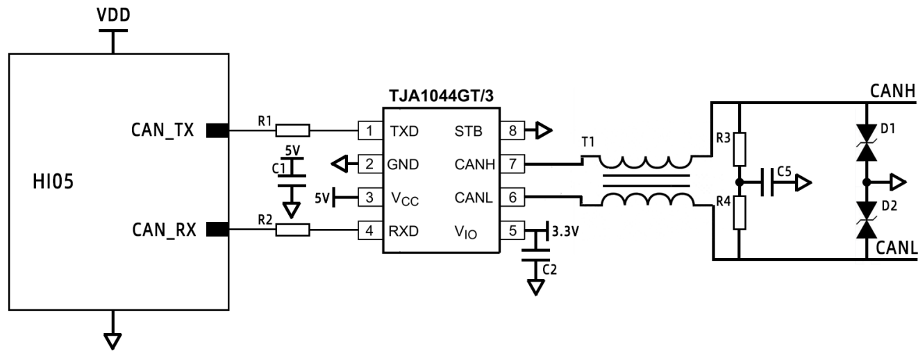
Figure7: HI05XX-MI0 CAN communication reference circuit
