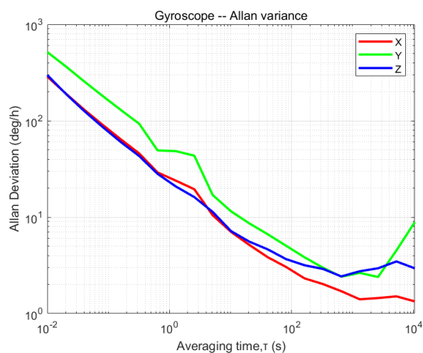
Figure4: HI13M0 Gyroscope Allan Variance
