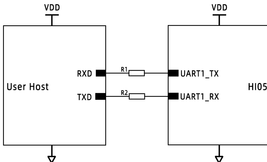
Figure6: HI05 UART communication ceference circuit
