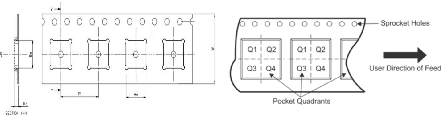
Figure22: Tape Dimension and pin 1
