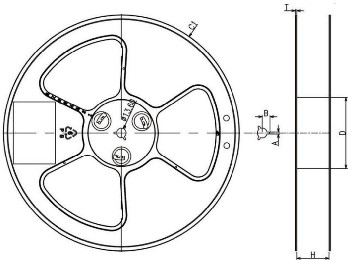
Figure23: Reel Dimension
