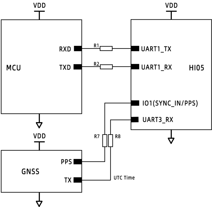
Figure10: HI05 GNSS-based synchronization
