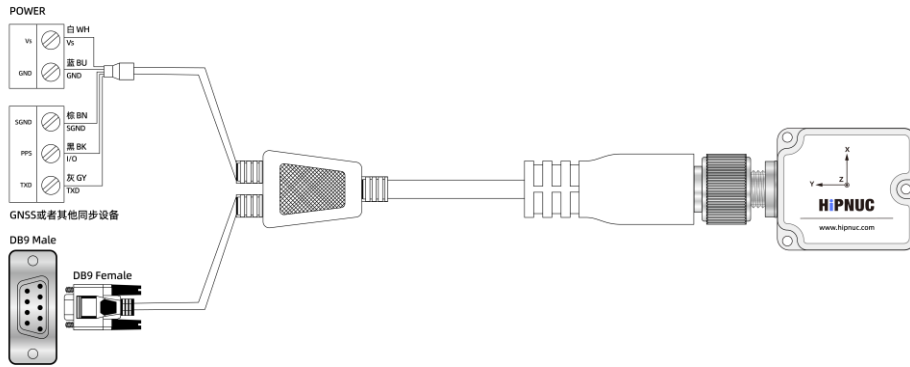
Figure 19: Wiring Diagram for UART (RS-232) PPS + GPRMC Synchronization with DB9 Connector
