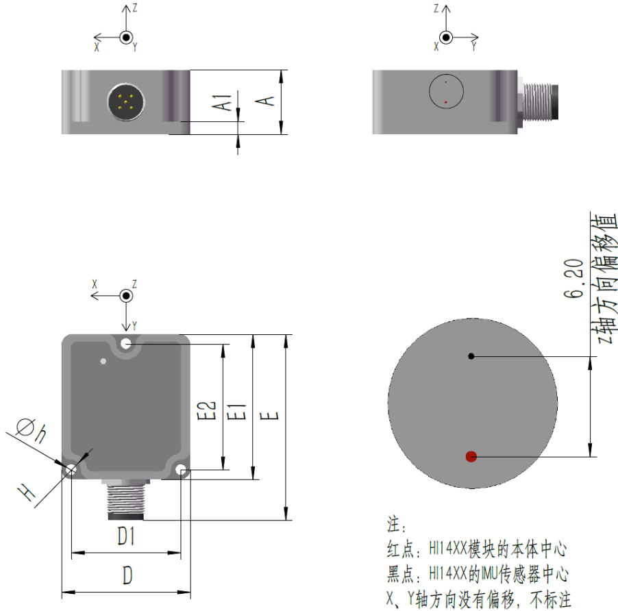
Figure 6: HI14 M12 Mechanical Dimensions
