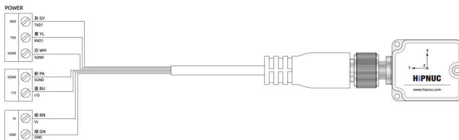
Figure 21: Wiring Diagram for UART (TTL / RS-232) Trigger Synchronization with Flying Leads
