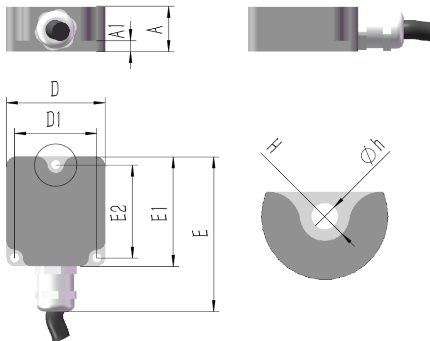
Figure 7: HI14 PG Mechanical Dimensions
